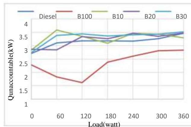
Figure 7: Unaccountable heat (Q) Vs Load
