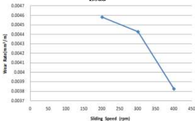
Figure 2: Variation of wear rate with change in Sliding Speed (when load applied is 30N)
