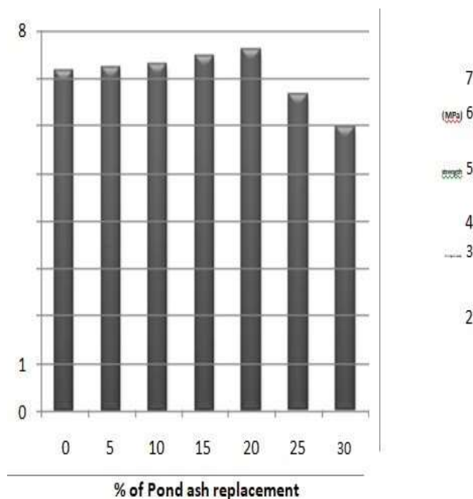
Figure 6. 28 days flexural strength of concrete with varying % of pond ash.
