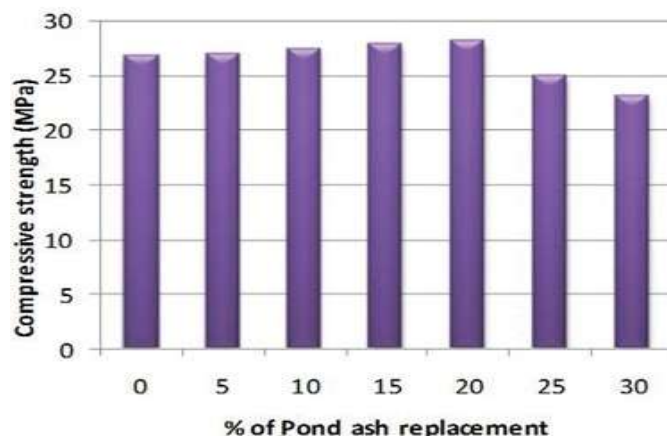
Figure 2. 7 days compressive strength of concrete with varying % of pond ash.
