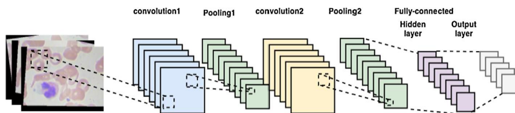
Figure 1: Architecture of ConVNet
