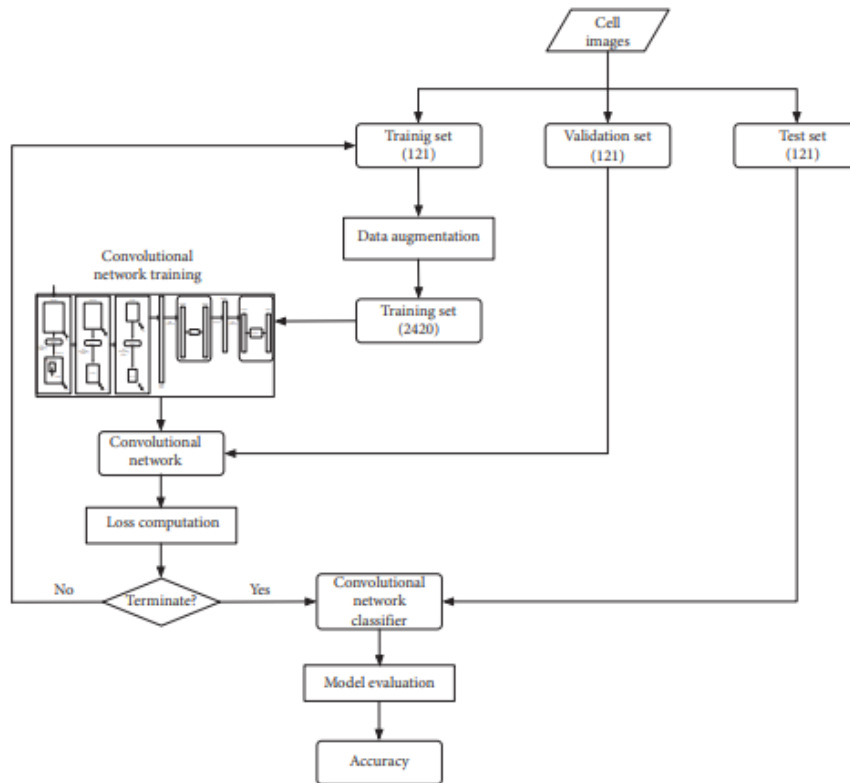
Figure 2: Image classification using ConVNet.
