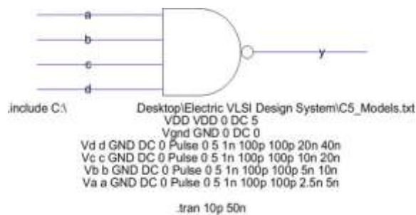
Figure 10. Icon of 4-input NAND gate and spice code
