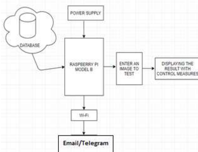
Fig10: Block Diagram
