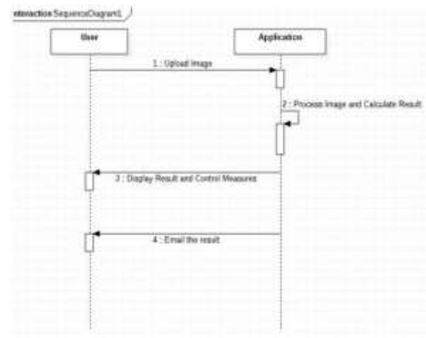
Fig14: Sequence Diagram
