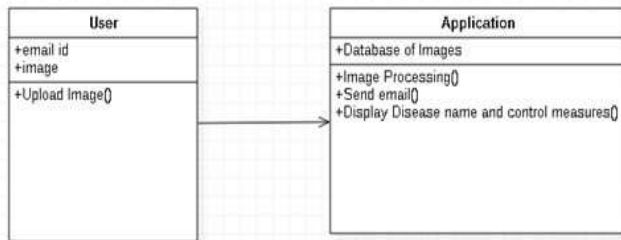
Fig12: Class Diagram
