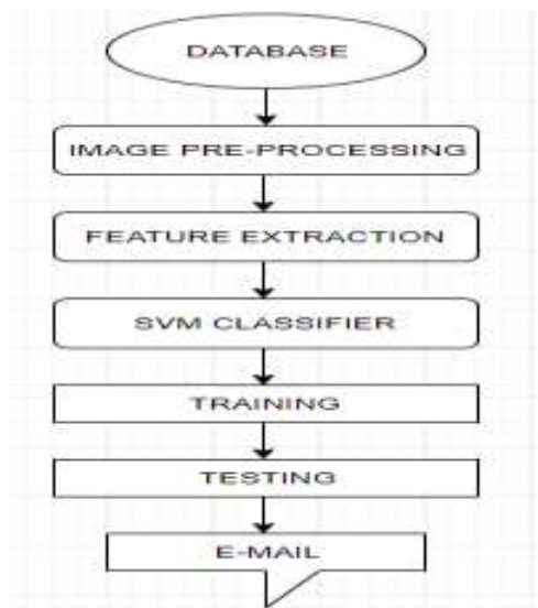
Fig11: Flow Chart
