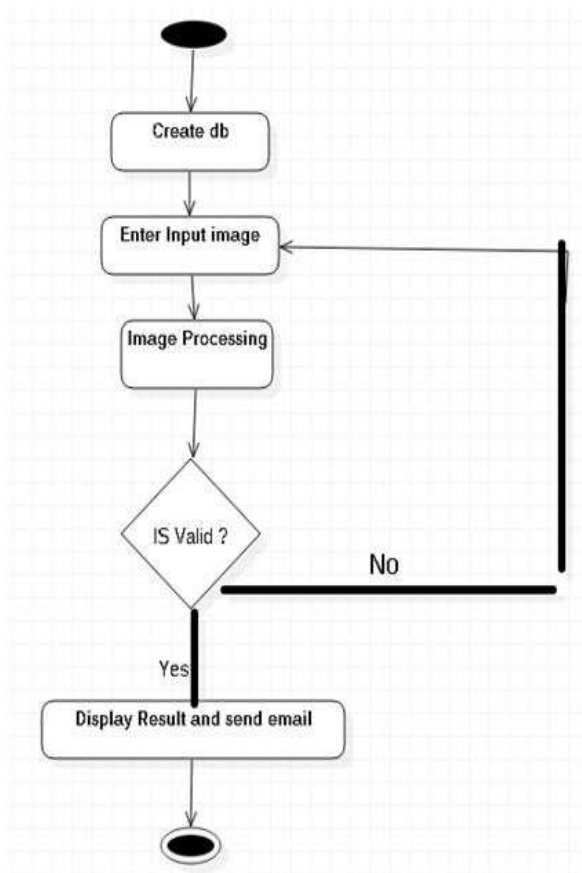
Fig13: Activity Diagram
