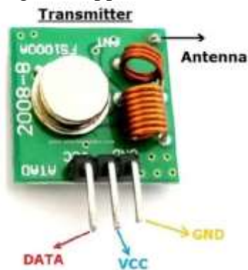
Fig-4: RF-Transmitter
