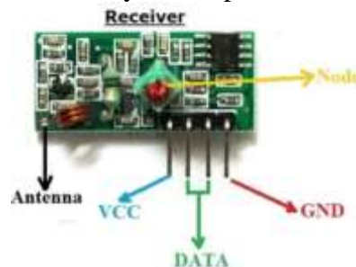
Fig-6: RF-Receiver
