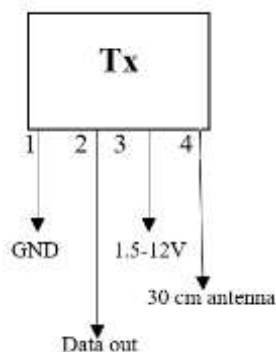
Fig-1: Pin diagram of Transmitter module.
