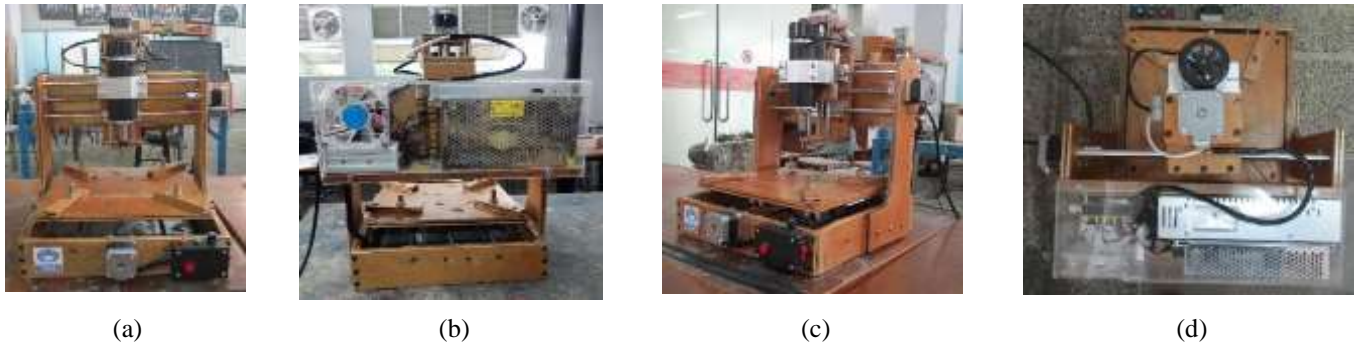
Figure 4: CNC machine display. (a)Front view (b)Back view (c)Corner right view (d)Top view
