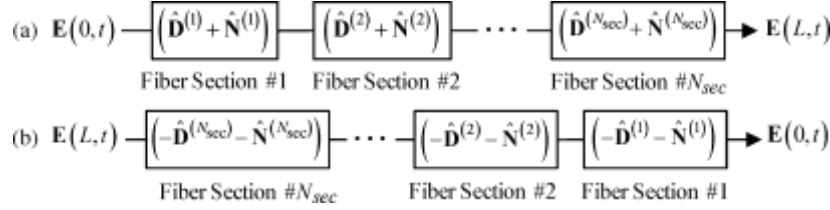
Fig. 21. (a) Forward and (b) backward propagation in a fiber channel modeled as the concatenation of N_{sec} sections.
