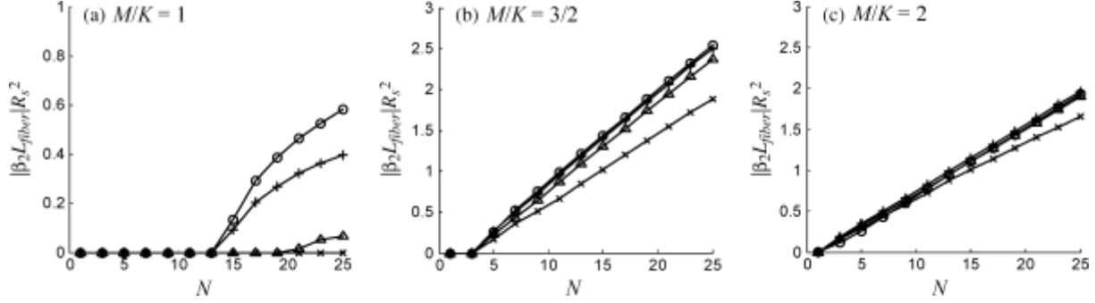
Fig. 5. Normalized residual CD versus equalizer length for oversampling rates of (a) 1, (b) 3/2, and (c) 2. For each plot, the curves denote: o: NRZ, x: 33% RZ, : 50% RZ, and : 67% RZ.
