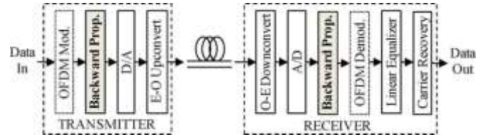
Fig. 20. Nonlinear compensation transmitter and receiver.
