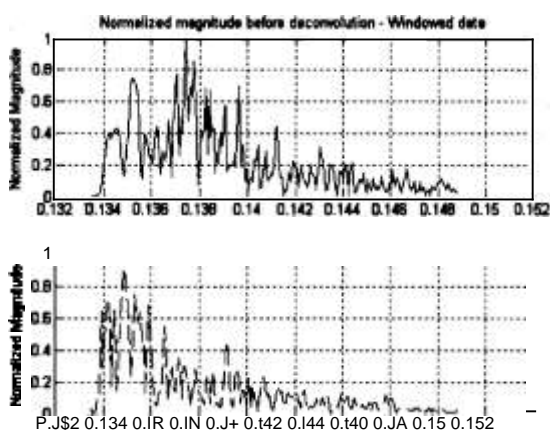
Figure 10: Normalized Magnitude of the windowed data before and after deconvolution
