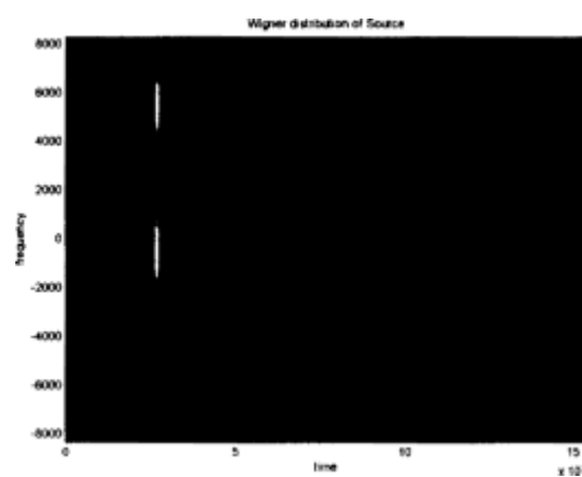
Figure 6: Wigner Distribution of the source at 0.035
