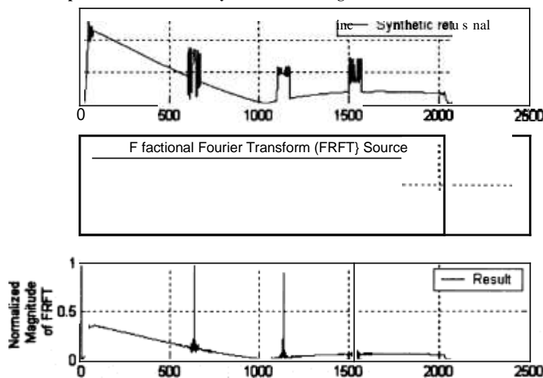
Experimental Results on Synthetic Data using Fractional Fourier Transform \alpha = 0.035
