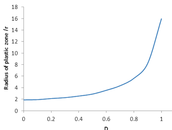
Fig. 6. The ratio of the radius of plastic zone to tunnel radius for different disturbance factors Diagram in Fig. 6 shows that by increasing disturbance factor, the ratio of the radius of plastic zone in the roof of tunnel increases and the most increase is in disturbance factors of 0.8 to 1. It also implies that for excavation of the tunnel No.2 of Kurdistan, the blasting method should not be
