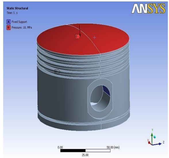
Fig.6 Loading and boundary conditions on piston
