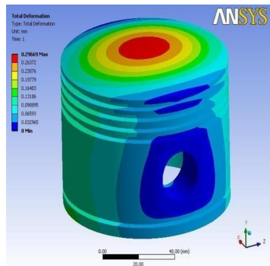
Fig.7 Total deflections on the piston head
