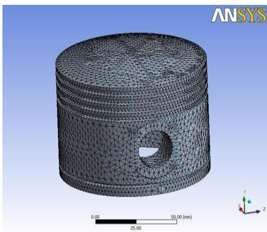
Fig.5 Meshed model of piston
