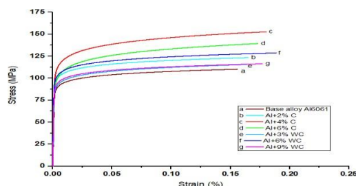
FIGURE 4. Effect of reinforcements on stress-strain curve
