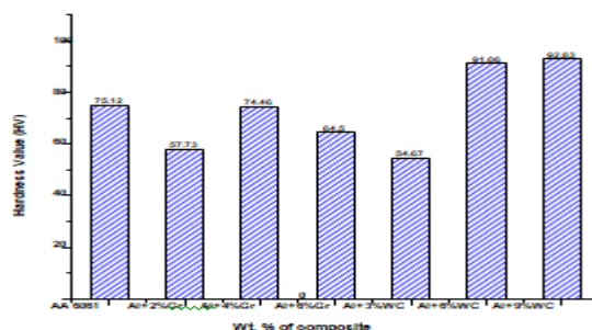
FIGURE 6. Hardness Values vs Wt% of Composite
