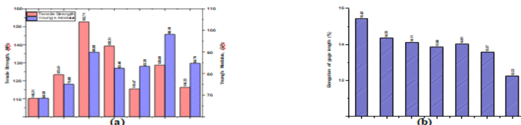
FIGURE 5. (a) Effect of reinforcements on Tensile Properties of composite (b) Percentage Elongation vs Wt % of composite
