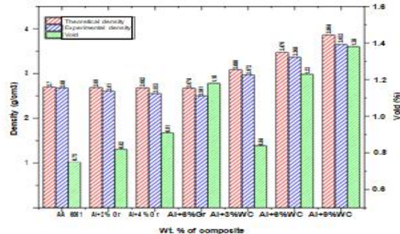
FIGURE 2. Density with Wt % of Composite
