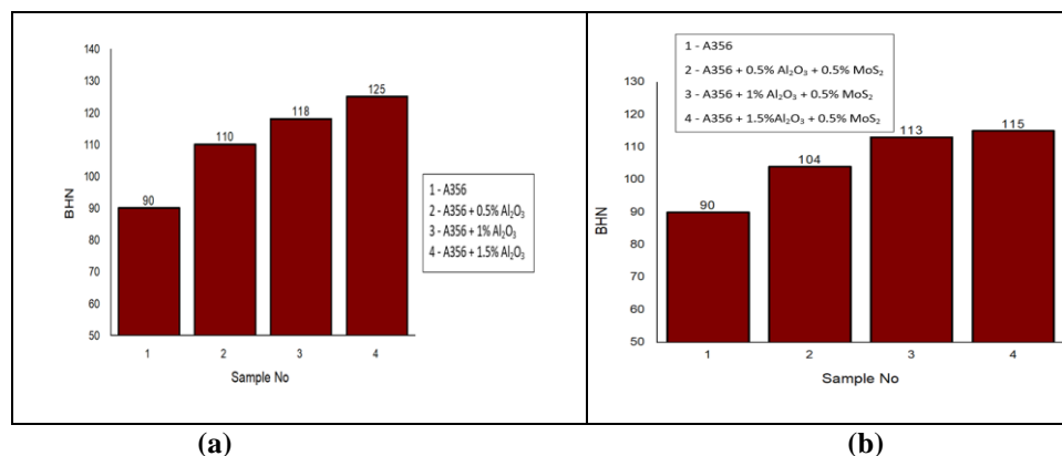
Fig 9: BHN v/s percentage of reinforcement
