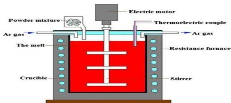
Fig. 1: Stir casting method
