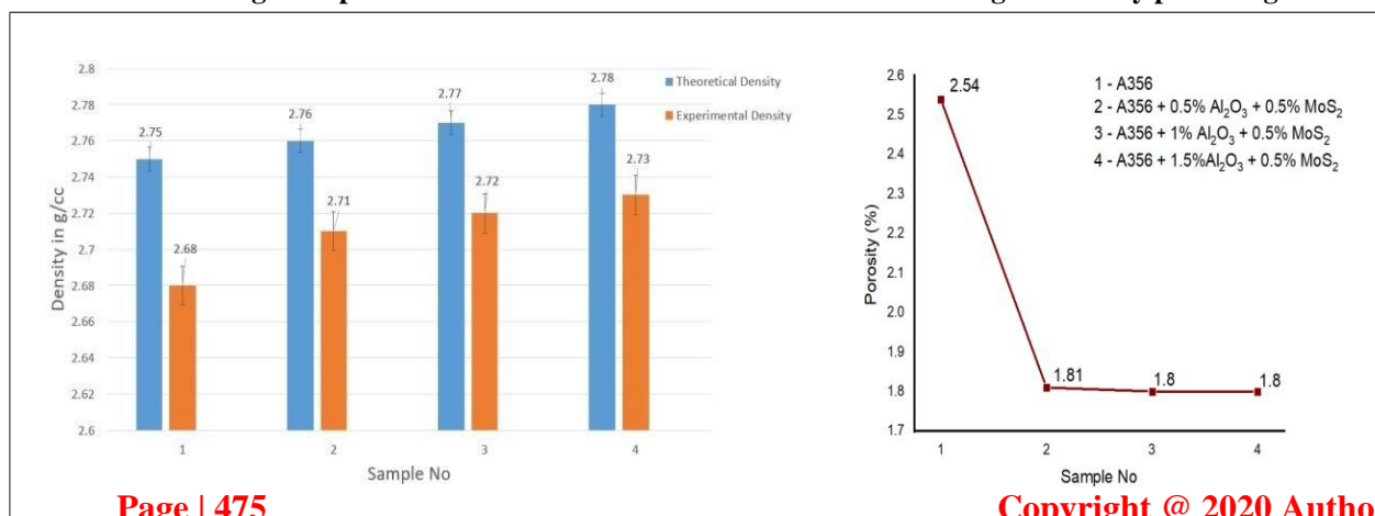
Fig 4: Experimental & Theoretical densities
