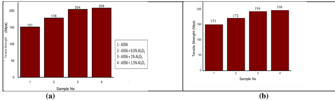
Fig 8: Tensile strength v/s percentage of reinforcement
