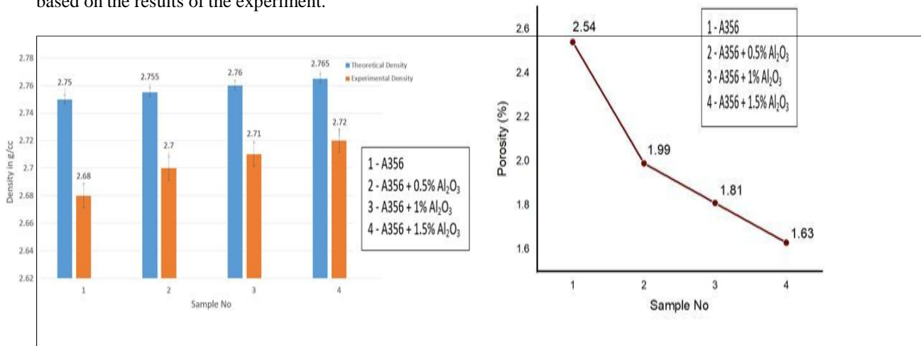
Fig 4: Experimental & Theoretical densities
