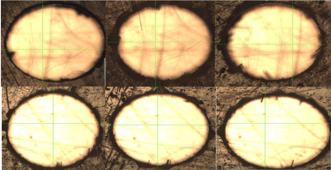
Figure 8 Photograph of circularity observation in CFRP (R2, R17, & R27) & GFRP (R1, R5, & R6) drilling.
