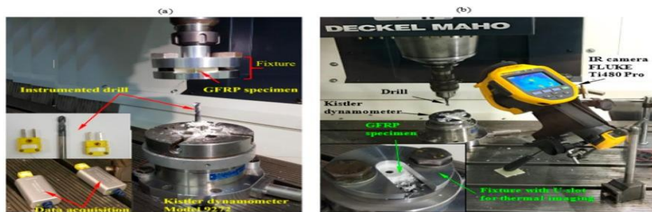
Figure 4 Experimental setup for measuring thrust forces and torque in drilling GFRP composites using CNC milling machine and Kistler dynamometer. The temperature was measured by: (a) instrumented drill with two thermocouples (b) IR camera (Khashaba U.A. 2021)
