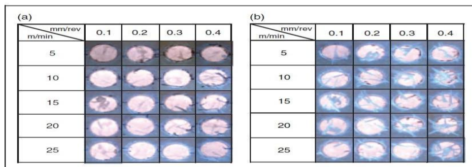
Figure 3 Photographs of the delamination observed in drilling GFRC (point angle: 118): (a) at entrance and (b) at exit (Kilickap 2010)
