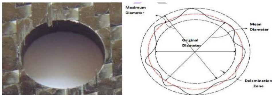
Figure 2 Drilled hole image & Scheme for measuring Delamination (Michael 2017)
