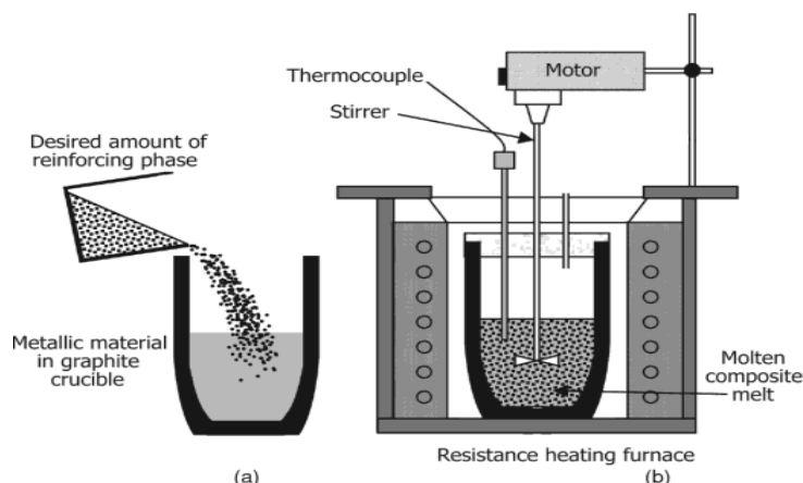
Figure 7. A schematic diagram showing (a) incorporation of reinforcing phase into matrix metallic material (b) the stir casting setup (Gupta and Sharon, 2011).
